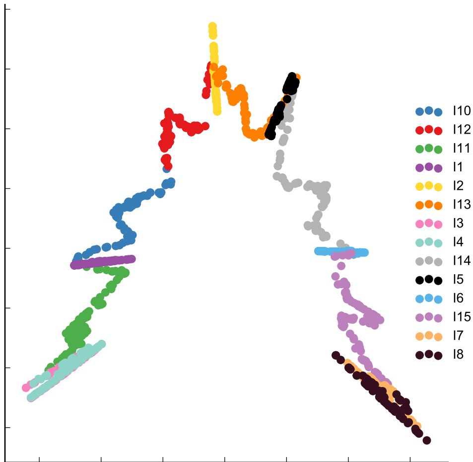
Spectral Embedding
