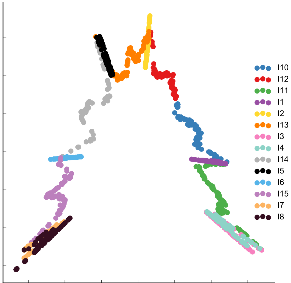
Spectral Embedding
